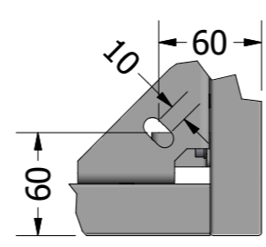
DETAIL A SCALE 1/4
